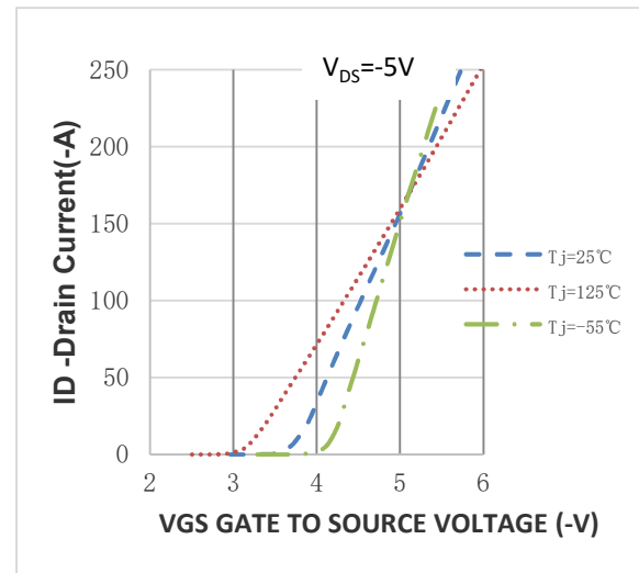
Figure 10. Transfer Characteristics
